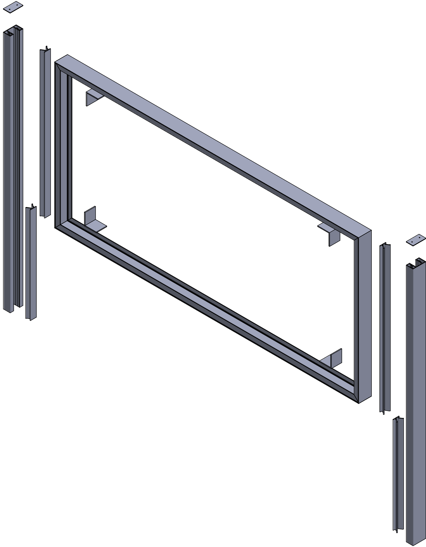
EXPLODED ISO VIEW
