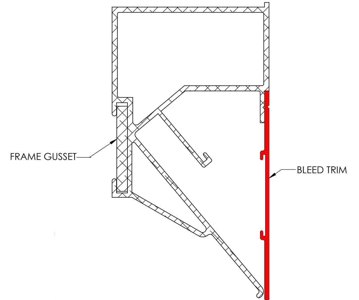
SECTION B-B ESP-FLEX INTEGRATED FRAME WITH BLEED TRIM SCALE 1 : 1
