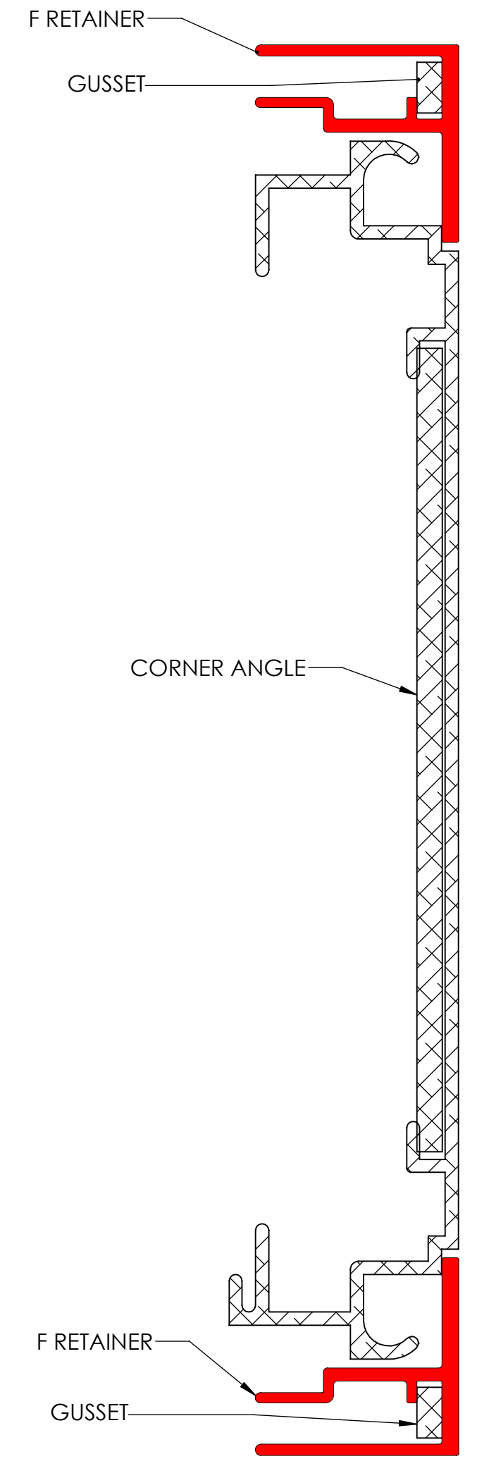
SECTION B-B ESP-DF HINGED FRAME WITH ESP-F RETAINERS SCALE 1 : 1
