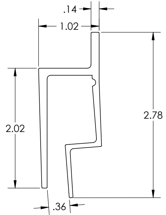
PROFILE VIEW
