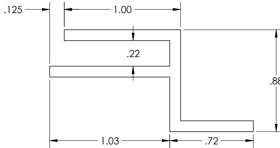
FRONT VIEW
