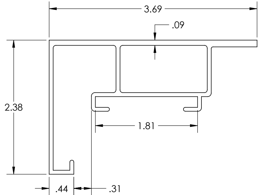
PROFILE VIEW
