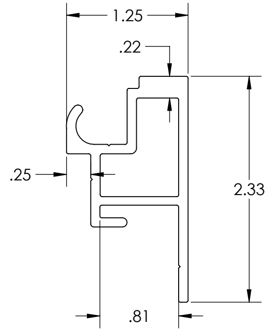
PROFILE VIEW
