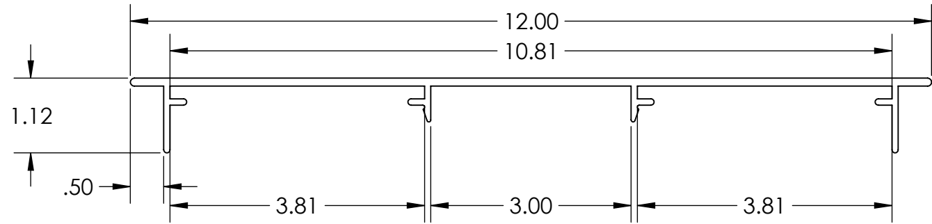
PROFILE VIEW
