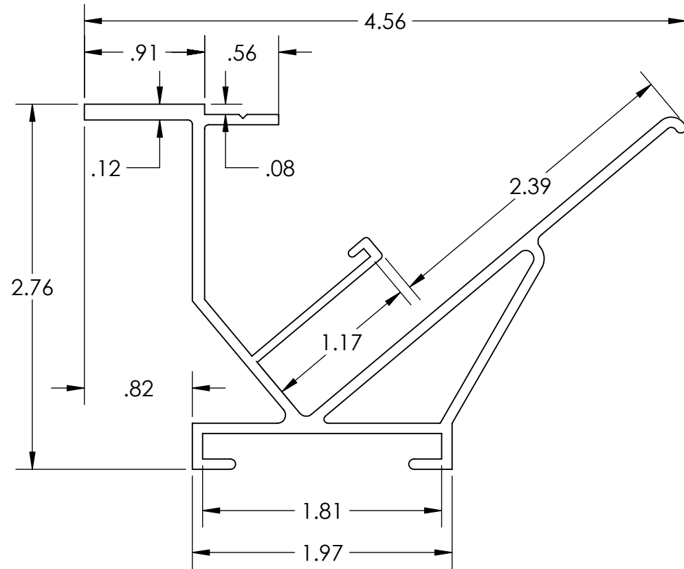
PROFILE VIEW
