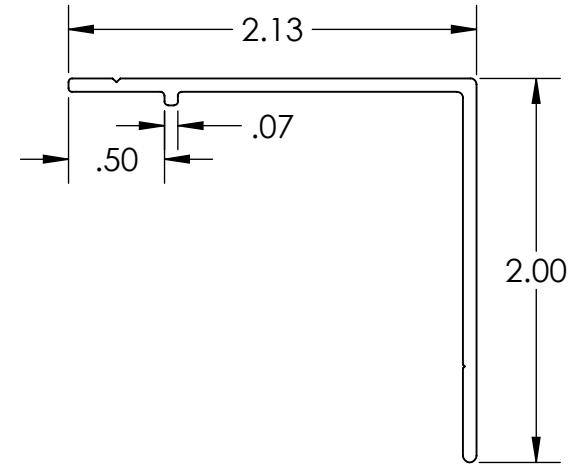
PROFILE VIEW
