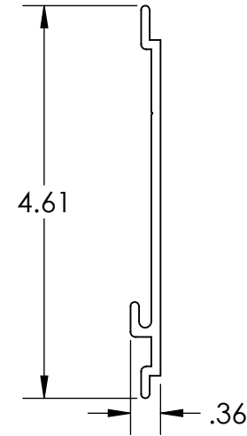
PROFILE VIEW
