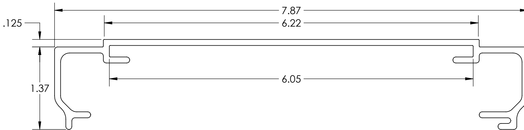
PROFILE VIEW
