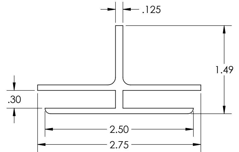
PROFILE VIEW
