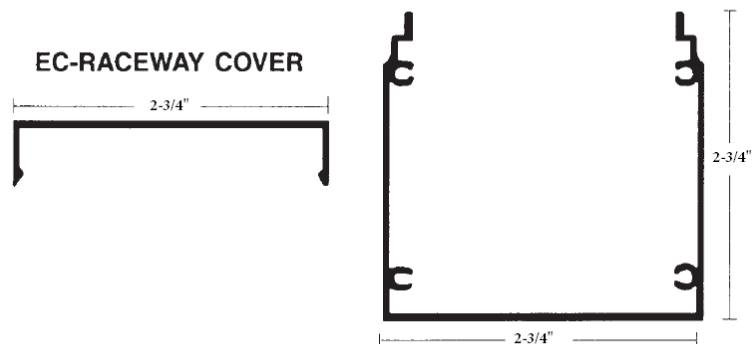
EC-Channel Letter Raceway
