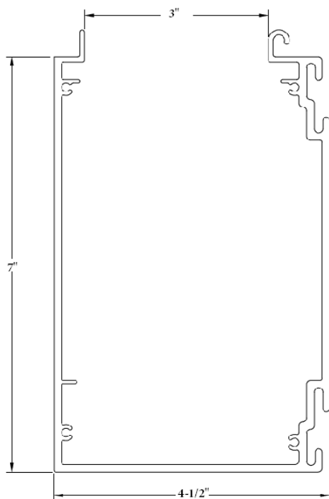
EC-Channel Letter Raceway
