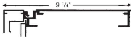
EC-S/F Hinged Frame w/ H-1 & FF-2 Retainers
