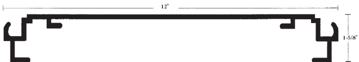
EC-12 Hinged Frame
