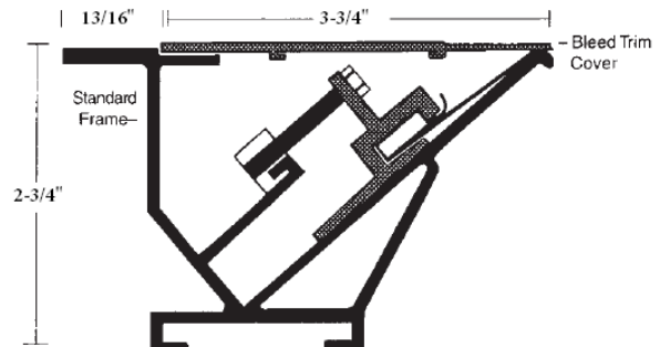
Standard Frame with Bleed Cover
