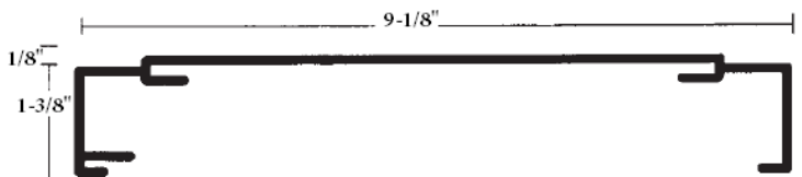
EC-D/F Standard Frame
