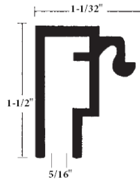
F Hinged Retainer
