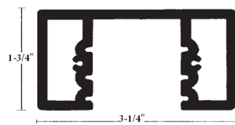
EC-3.25 Rectangular Post
