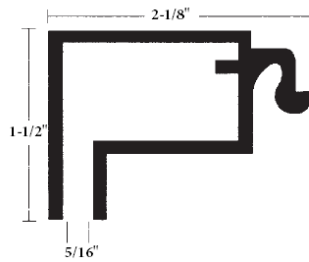
FF Hinged Retainer
