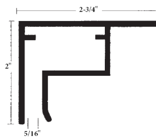
EC-Xtra Hinged Retainer
