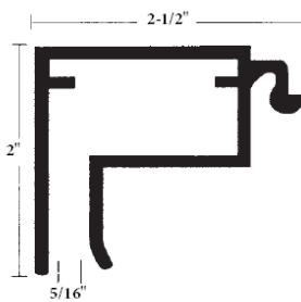
FF-2 Hinged Retainer
