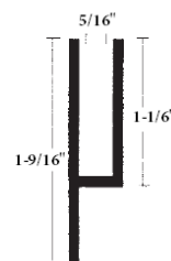
H-1 Retainer
