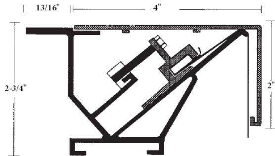
Standard Frame with Standard Cover
