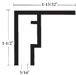
F Retainer
