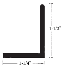
LF Retainer
