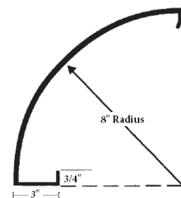
8" Radius Quarter End
