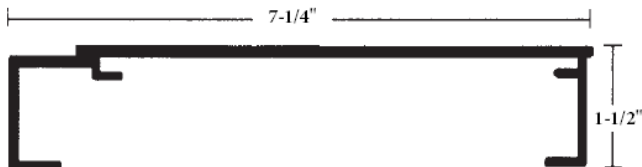
EC-S/F Standard Frame
