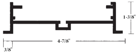
EC-Lamp Raceway
