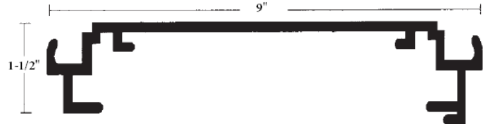
EC-D/F Hinged Frame
