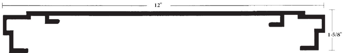
EC-12 Standard Frame
