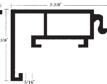
EC-Xtra Hinged Retainer
