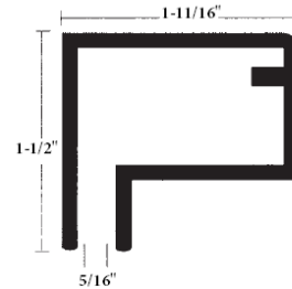
FF Retainer Short
