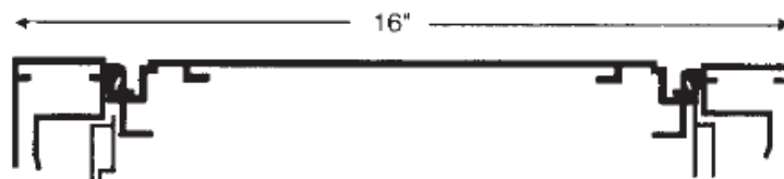
EC-12 Hinged Frame w/ H-1.5 or H-1 & FF-2 Retainers
