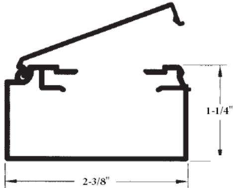
EC-Socket Raceway
