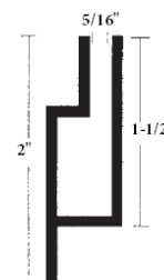
H-1.5 Retainer
