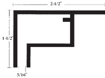
FF Flat Face Retainer
