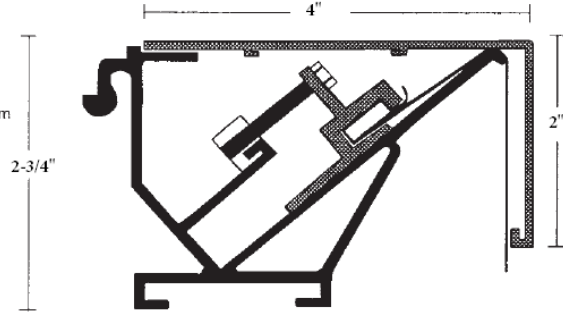
Hinged Frame with Standard Cover
