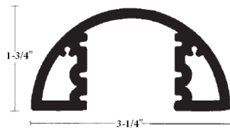
EC-3.25 Radius Post
