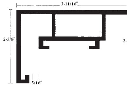
EC-Xtra Wide Retainer
