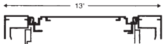
EC-D/F Hinged Frame w/ H-1.5 or H-1 & FF-2 Retainers
