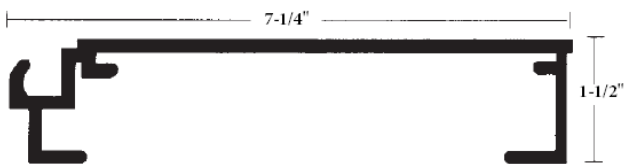
EC-S/F Hinged Frame
